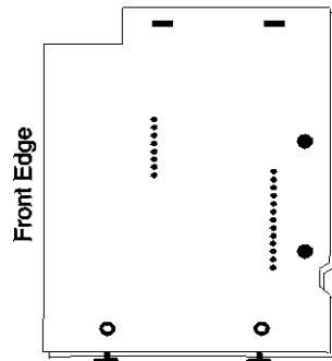
Support Panel (1 ea.)
